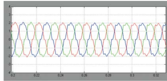
Fig. 5. Line Current of the SEIG with Multi level inverter fed WECS
