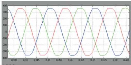
Fig. 3. Generated Output Voltage of SEIG
