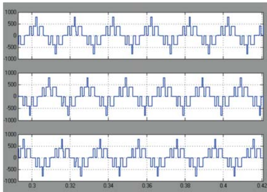
Fig. 4. Line Voltage of the SEIG with Multi level inverter fed WECS
