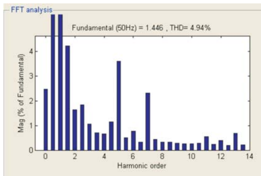
Fig. 9. Line Current of the SEIG with Z-Source Inverter fed WECS
