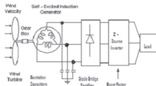
Fig. 1. Proposed Impedance Source Inverter based Wind Power Generation System
