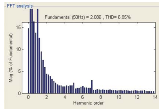
Fig. 6. FFT Analysis of the SEIG with Multi level inverter fed WECS
