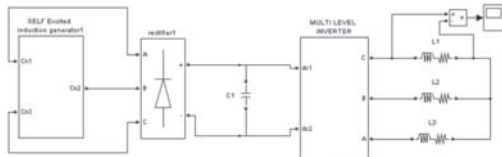
Fig. 1. Simulation Model SEIG with Multi Level Inverter fed R – L Load System
